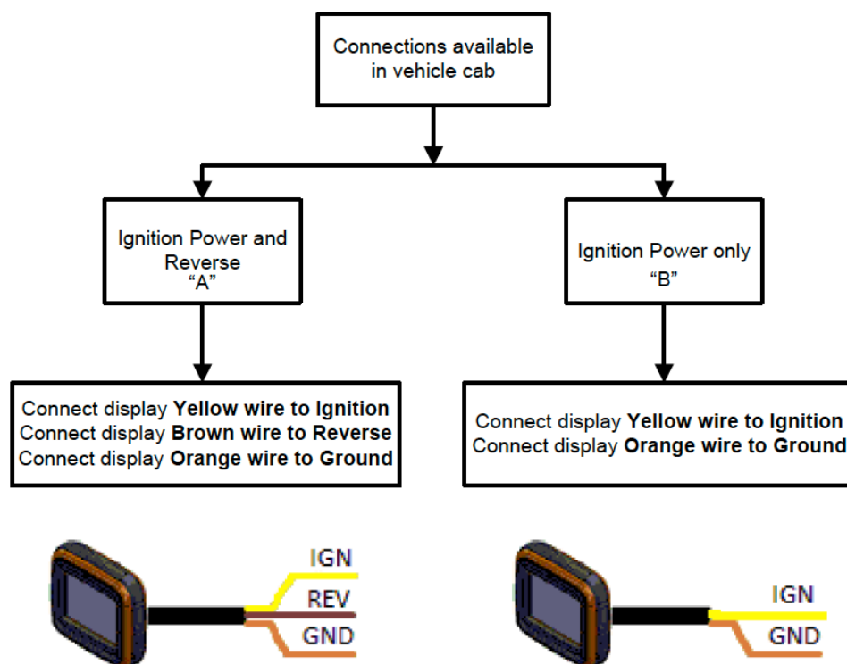
Figure 1. Electrical Connections
