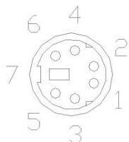
CONNECTOR FACE VIEW
